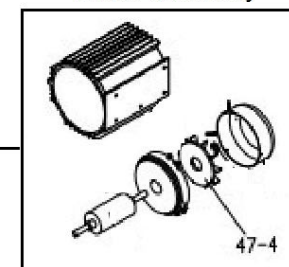
Motor assembly
