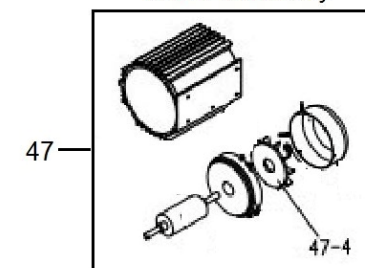
Motor assembly
