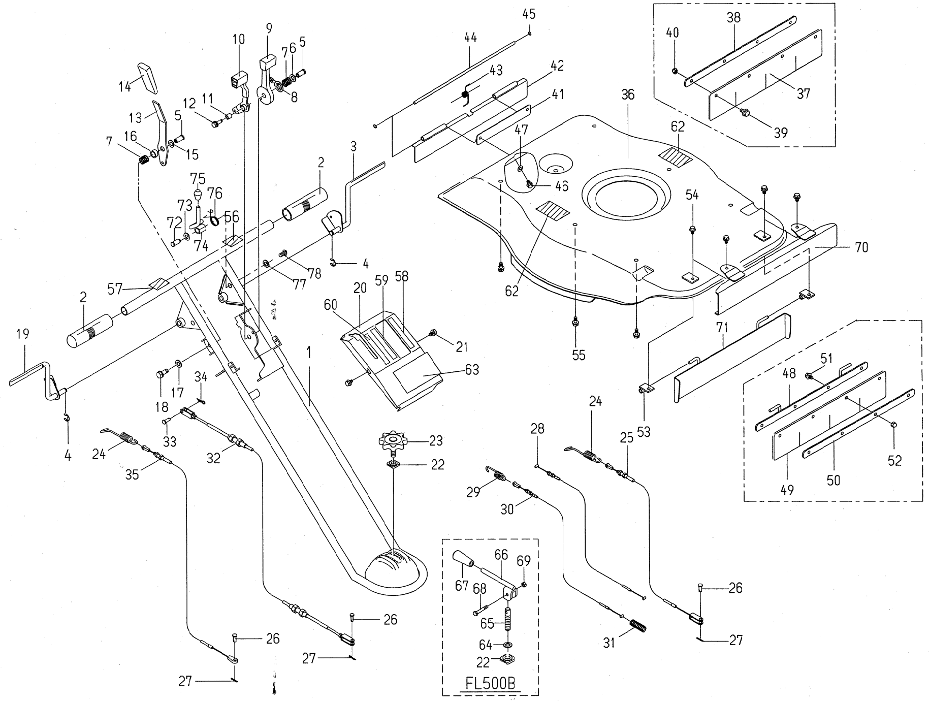
FIG.1 HANDLE & ROTARY COVER
