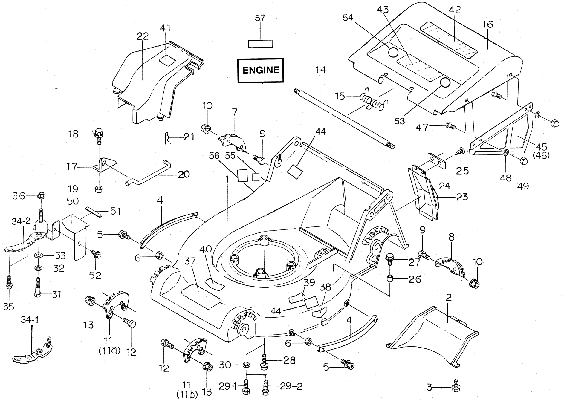
Fig 3 Safety Cover
