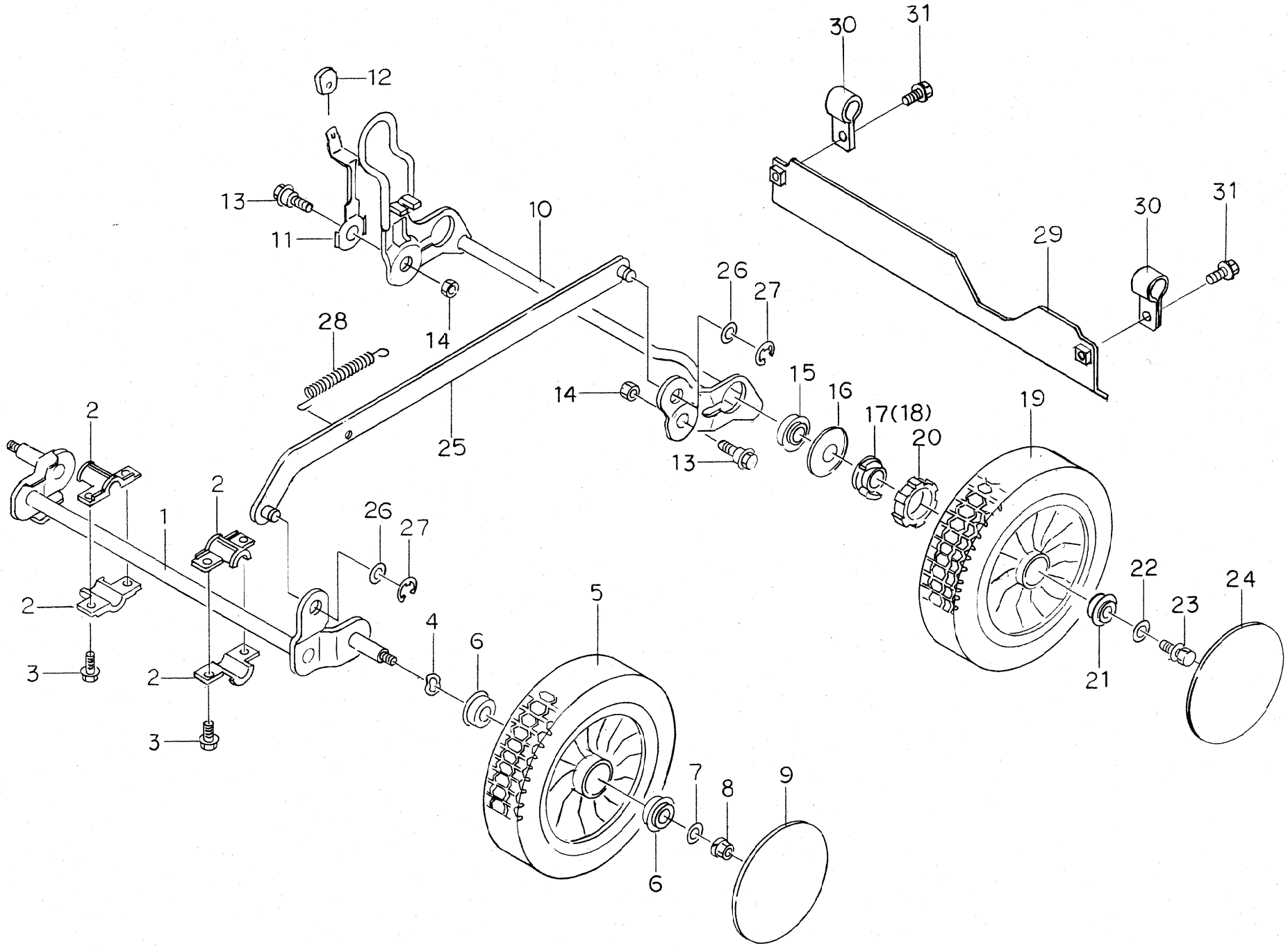
Fig 4 Wheel (GR532)
