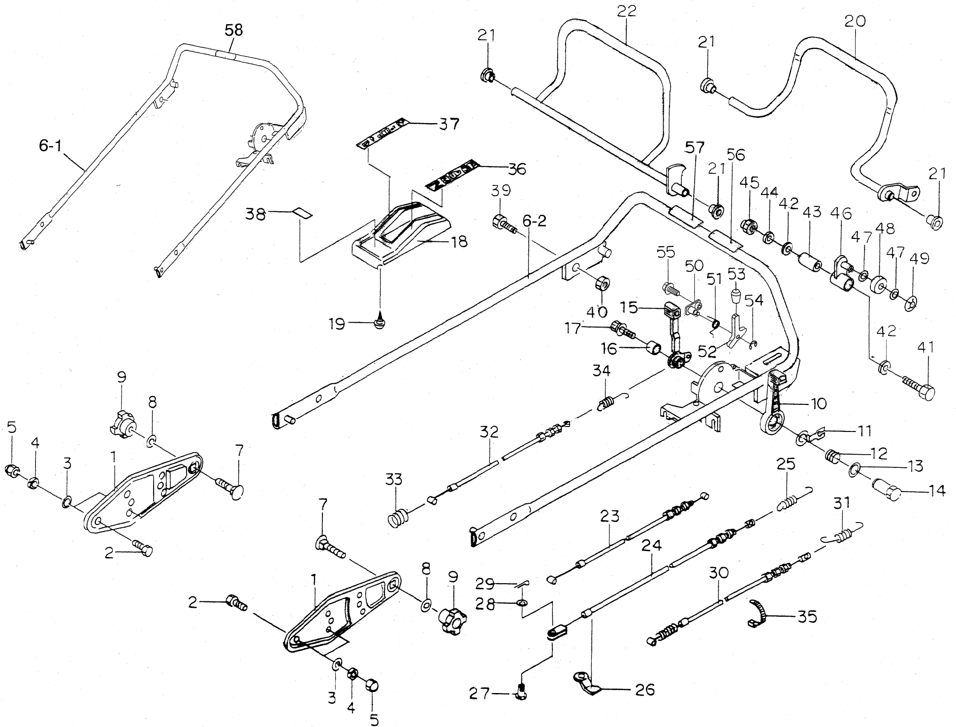
Fig 5 Handle
